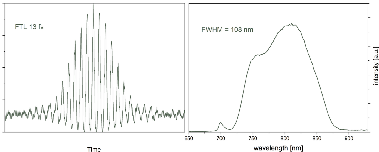
Typical autocorrelation and spectrum measurement of a 13 fs pulse
