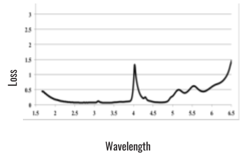
IRF-S-100 Attenuation Spectrum
