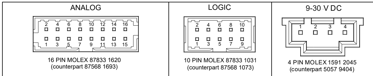
Figure 2. Pin configurations for SLD-uCS control ports and power supply connectors.
